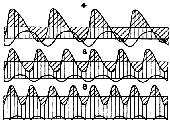
Torque Curves for Four, Six and Eight Cylinders.
